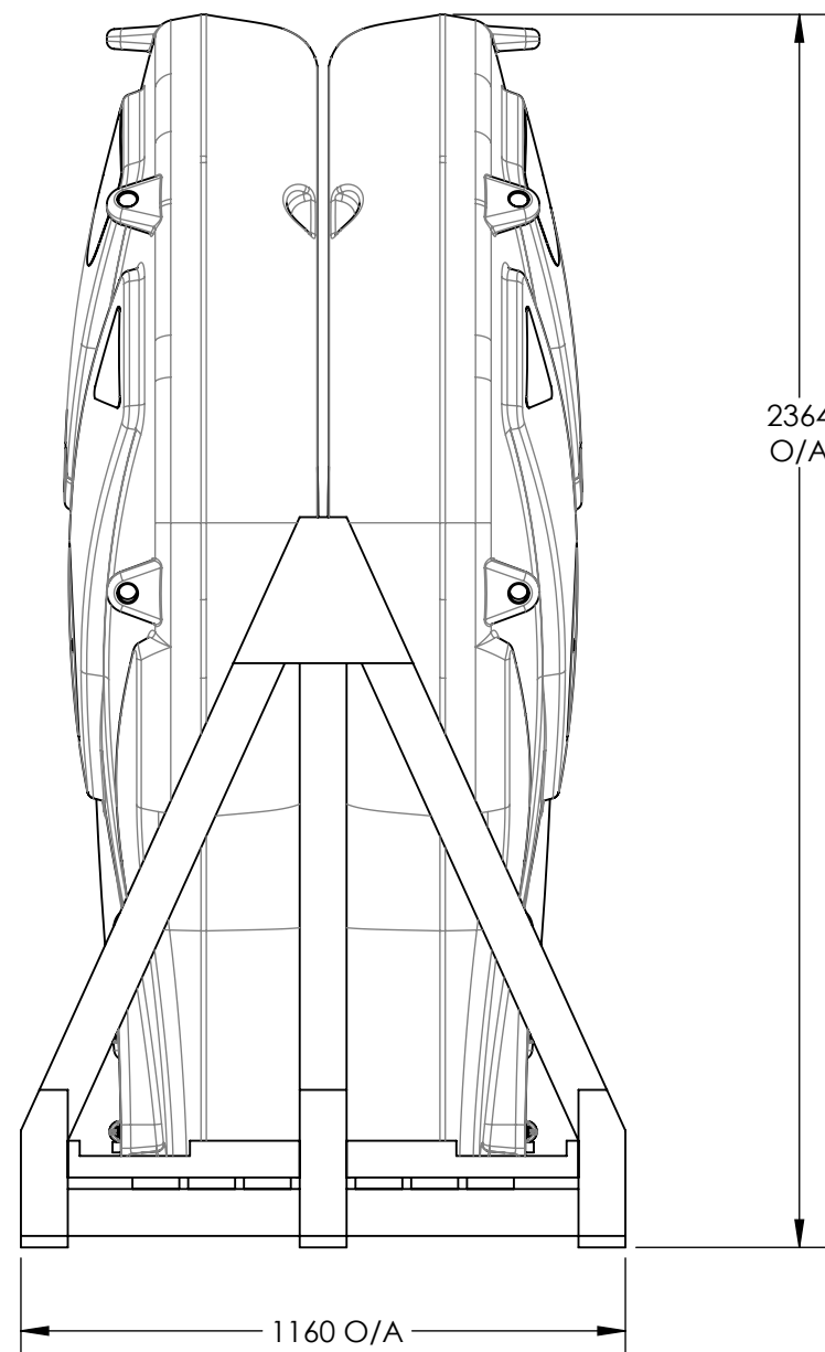
SIDE VIEW
