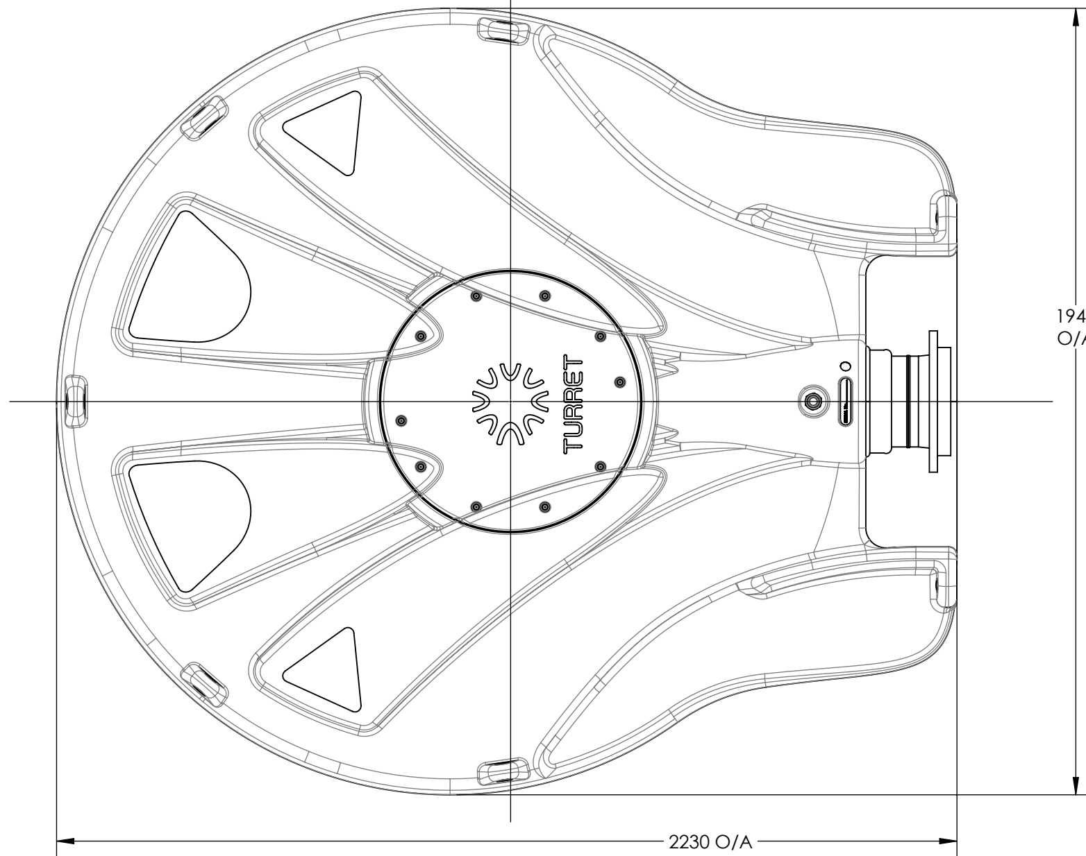
PLAN VIEW
