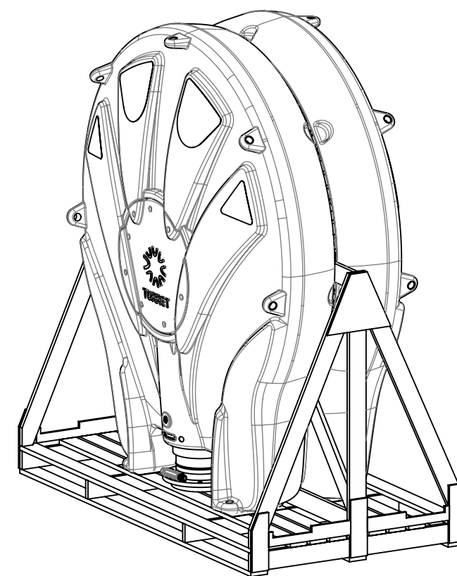
PICTORIAL VIEW
