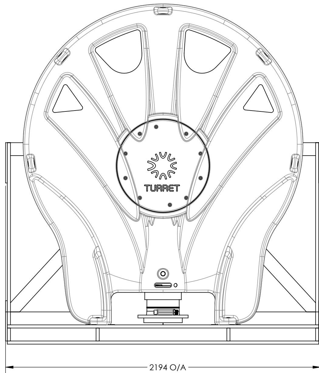
FRONT VIEW
